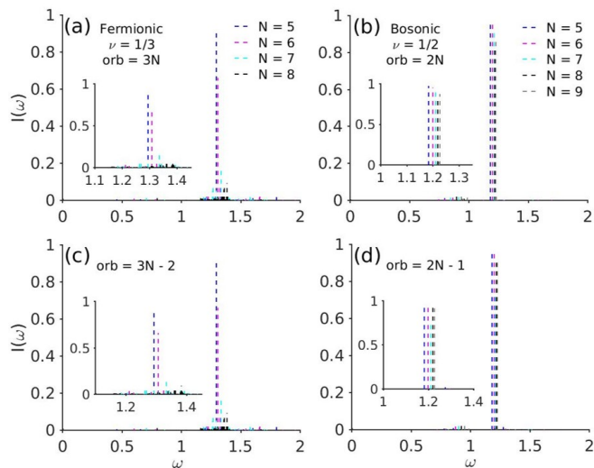
FIG. 3. A bird's-eye view of (a) and (c) fermionic I_-(\omega) with 3N and 3N - 2 orbitals and of (b) and (d) bosonic I(\omega) with 2N and 2N - 1 orbitals for N particles on disk geometry. For all sizes, we recovered up to 97% of the total weight for fermionic case and up to 99% for bosonic case. In all cases, the graviton absorptions stand out against the background noise.
