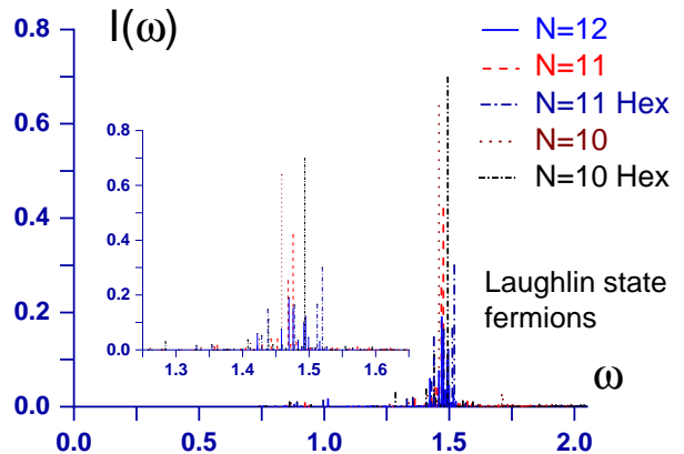
FIG. 1. A bird’s-eye view of the I_-(\omega) from fermionic Laughlin ground state at \nu = 1/3 for various sizes and geometries (Hex stands for hexagon geometry; square geometry otherwise). The graviton response can clearly be seen. The inset shows more details near energies where the response is strong. For N = 10 and 11 we recovered over 97% of the total weights. Unlike the case of bosons (shown below) the ‘‘background noise’’ a seems to be stronger for fermions, which are also computationally more costly than bosons. Accordingly, for N = 12 we recovered 90% of the weight over 87% of which is in the window of the inset. The rest, at higher energies, appear to be background noise. For example, we recover over 99% of the weight for 10 electrons. However, no significant peaks other than those shown in the inset was seen. The total weight in the inset is only 87% of the total weight. In other words about 12%, at higher energies, is just background noise.
