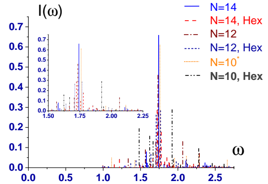
FIG. 6. The spectral function I(\omega) for the MR state of bosons with even number of particles at \nu = 1 .
